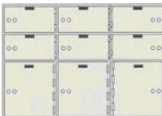
AX-9 (170 lbs.) 6 openings ea. 5" x 10" 3 openings ea. 10" x 10"
